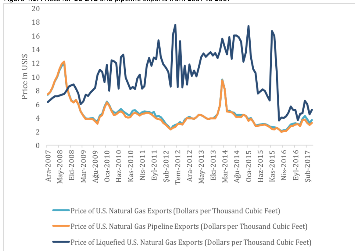
Figure 4.1: Prices for US LNG and pipeline exports from 2007 to 2017
