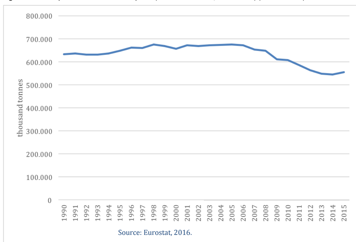
Figure 3.2 - European Union oil consumption (thousand tonnes, 1990-2015) (28 countries)
